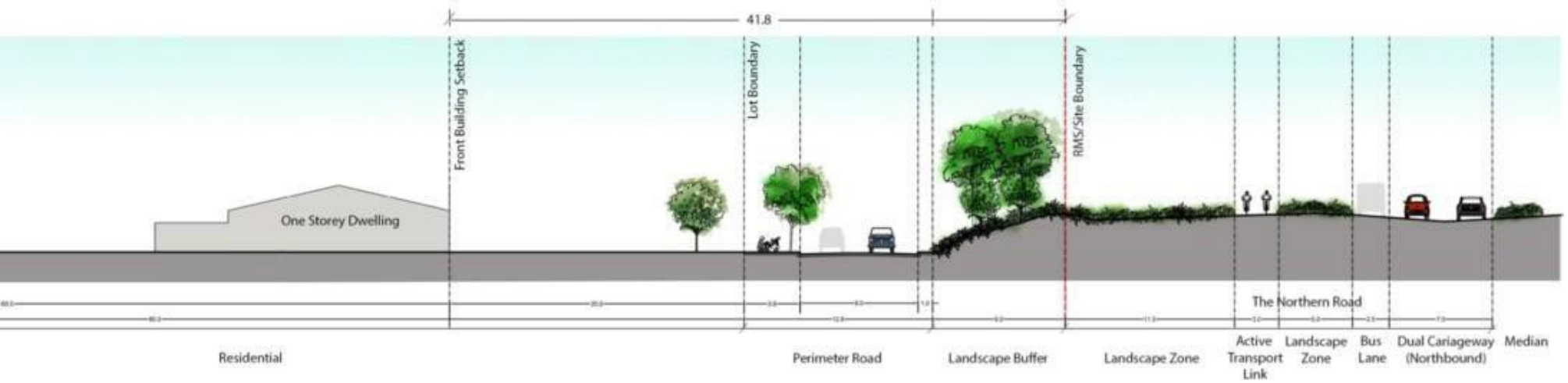
Figure E7.X Cross Section of Lots fronting The Northern Road, Internal Perimeter Road and The Northern Road road reserve.
