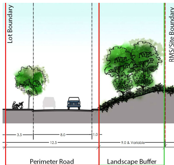
Figure E7.70: The Northern Road Indicative Interface
