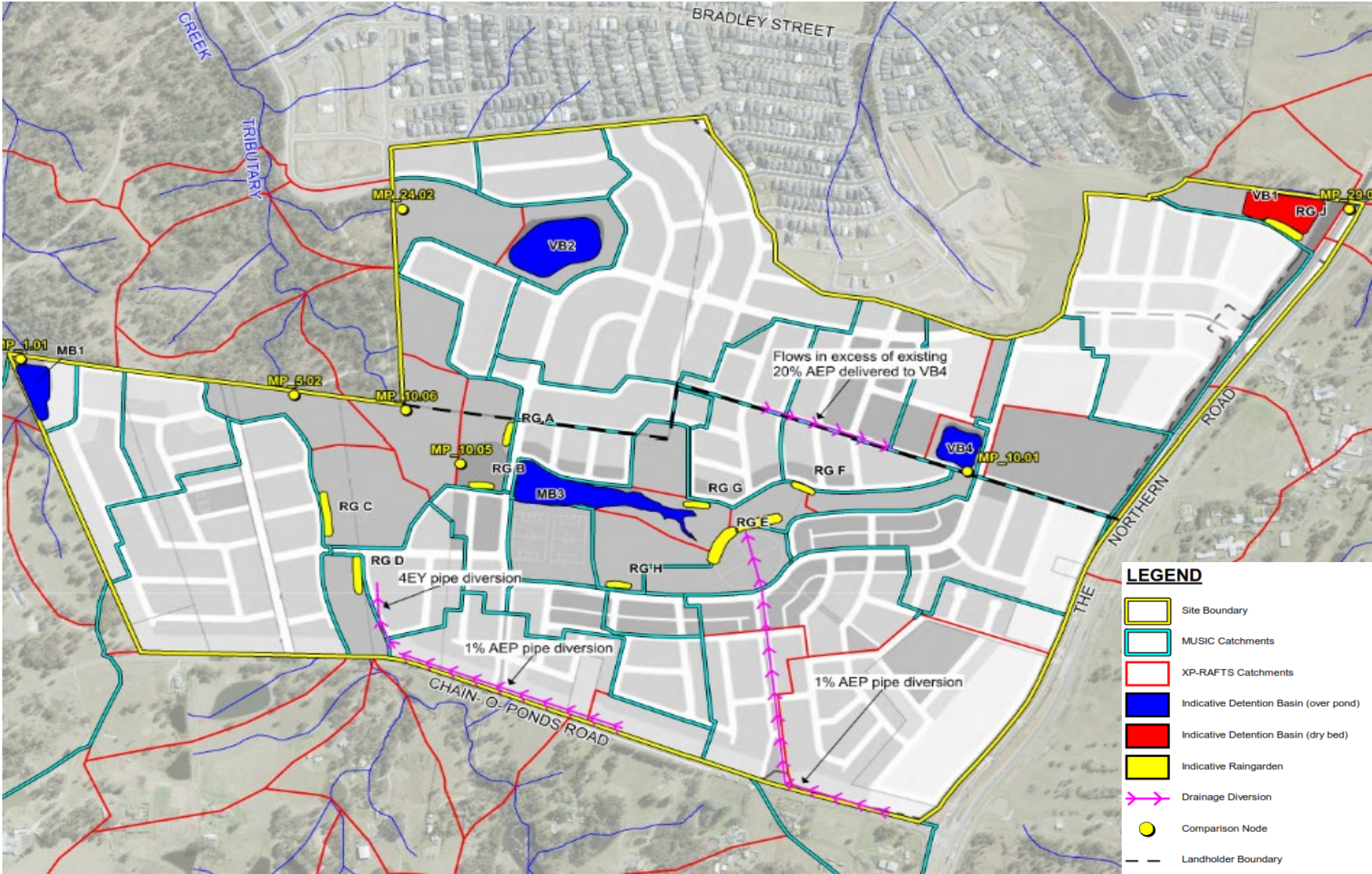
Figure E7.63: Indicative Water Cycle Management
