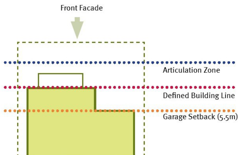
Figure E7.84: Setbacks and Articulation
