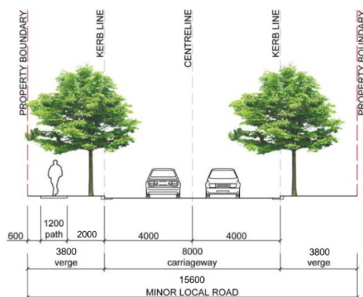
Figure E7.73: Minor Local Road
