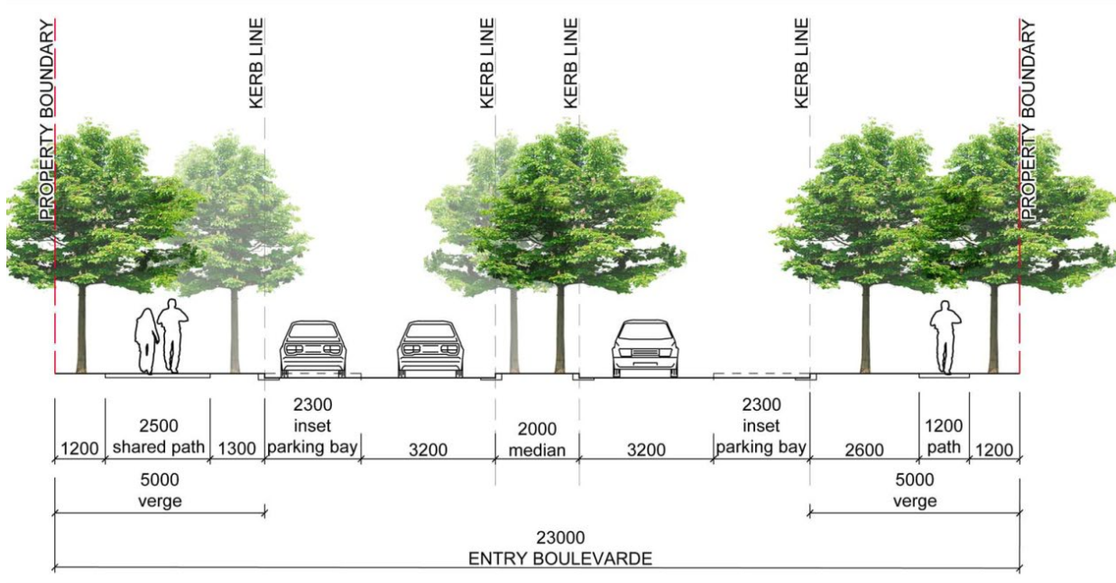
Figure E7.71: Entry Boulevard Roads
