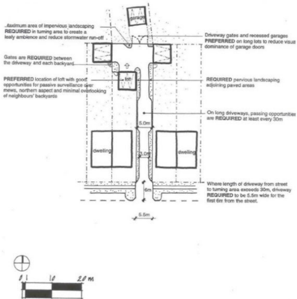
Figure E7.81: Shared Driveway - Design Principles
