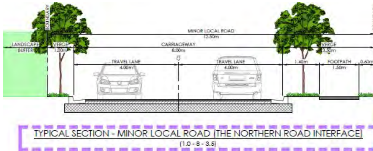
Figure E7. 66 The Northern Road indicative interface
