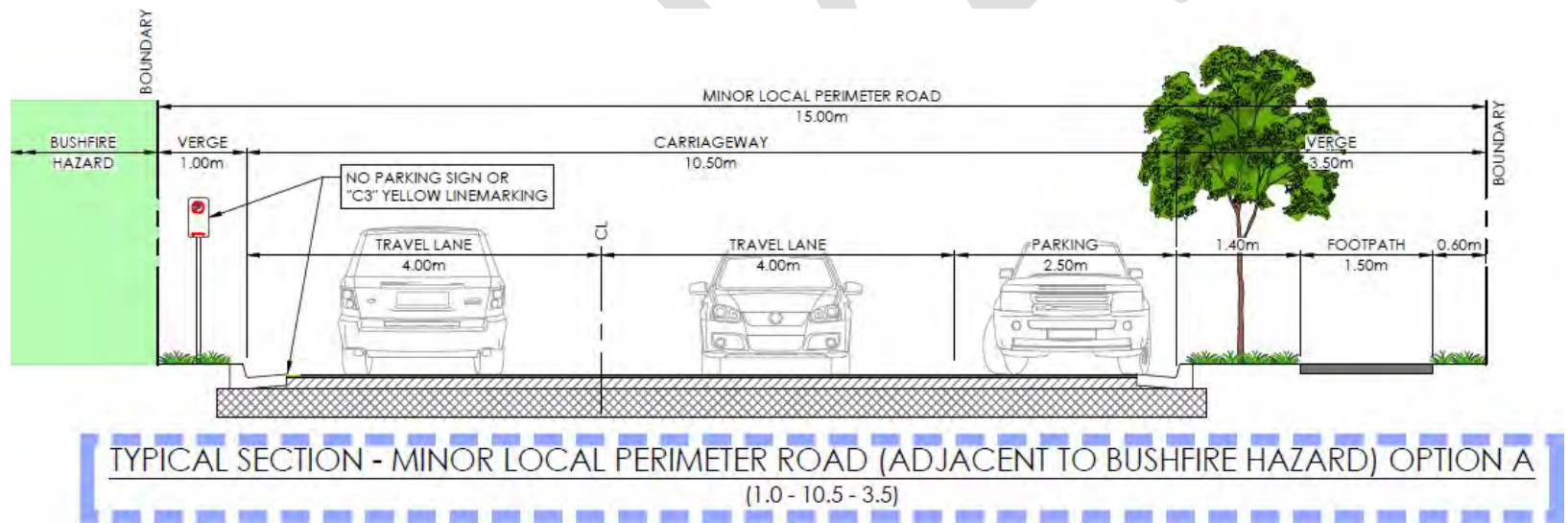
Figure E7.75 Minor Local Perimeter Road (Adjacent to Bushfire Hazard) Option A
